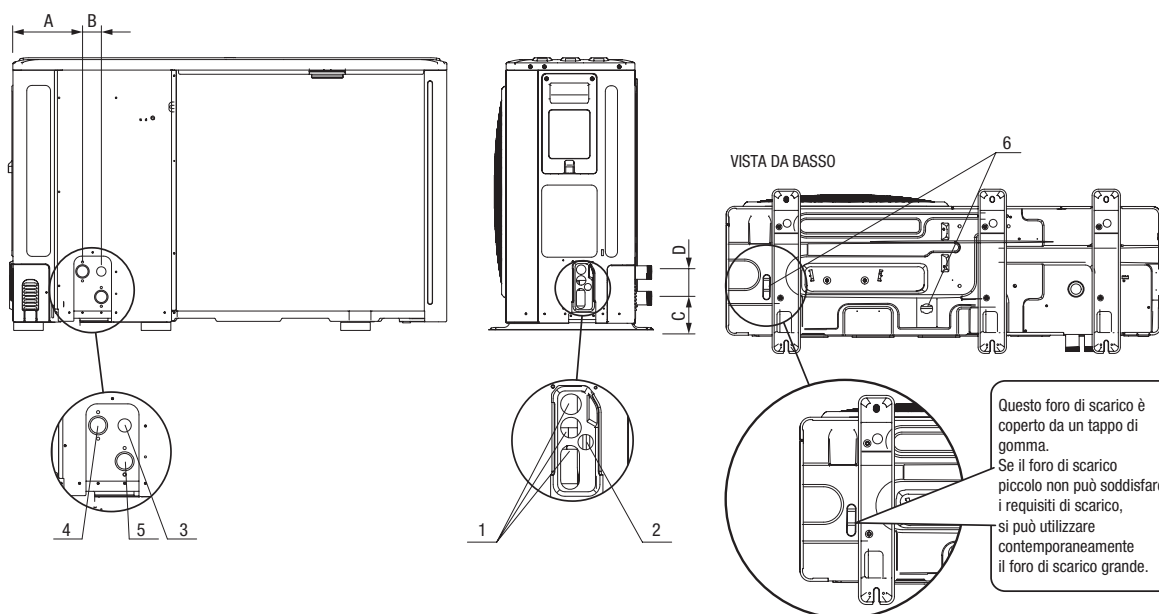
HYDRO UNIT M 008
